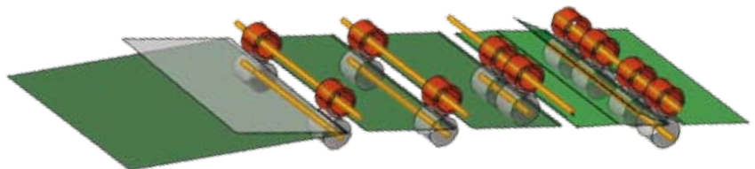
Figure 1. 3D CAD model of a typical printer paper flow path. The paper is pulled into the printer (‘nipped’) between a rotating upper rubber roller (the drive) and a stationary, spring-loaded lower plastic roller (the driven, or idler). During the printing process the paper is conveyed through a series of these rollers, with baffles and stationary guides (not shown) directing its path.
